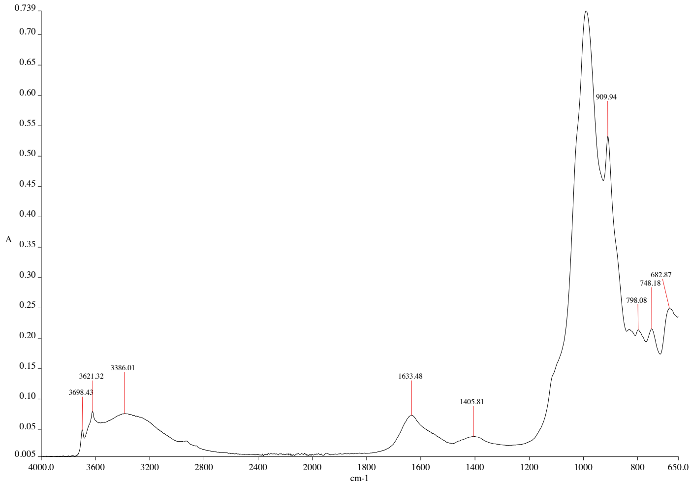
Data Fig 49 FTIR spectra for sample from interior of copper-alloy cylindrical container <S24>
