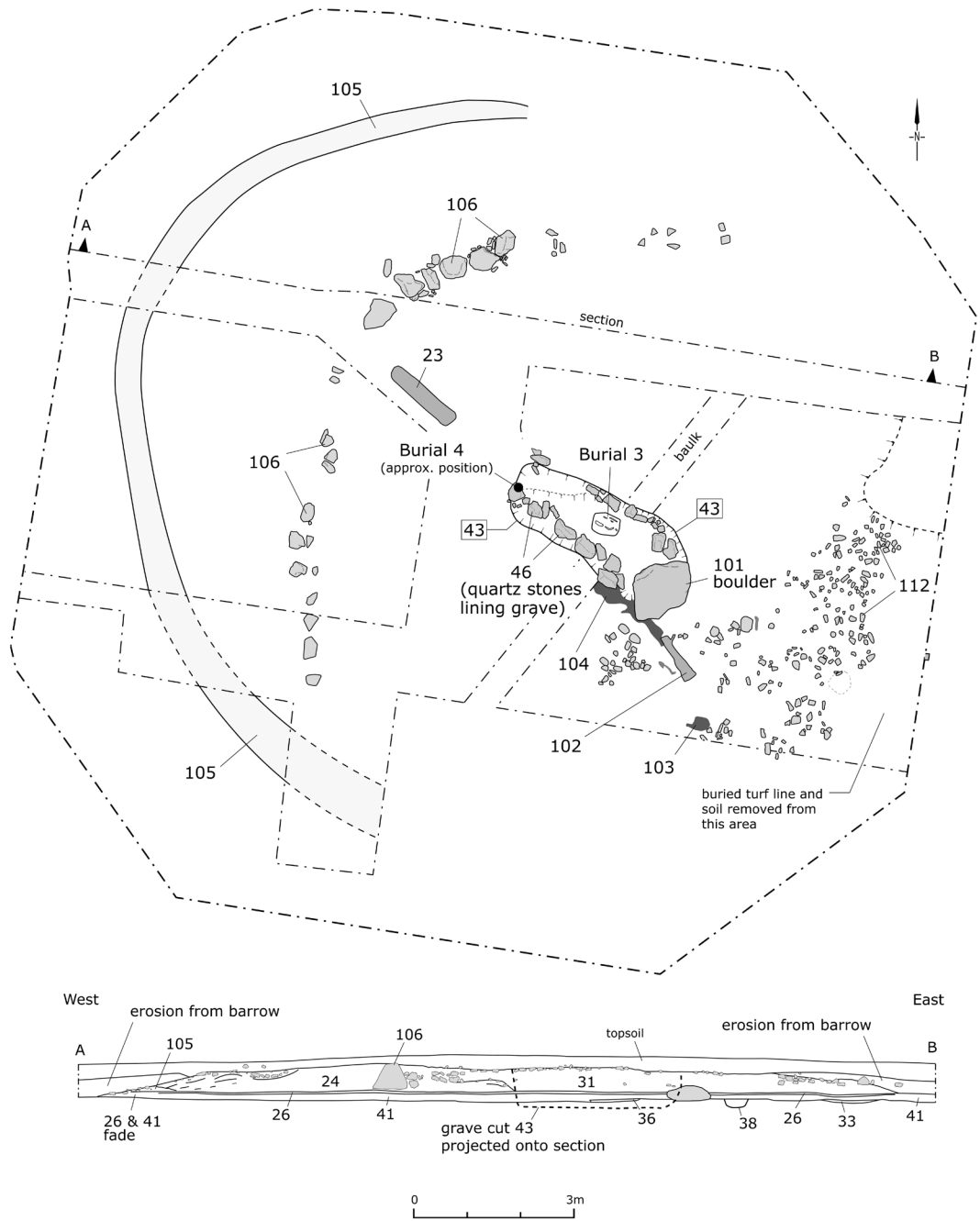
Fig. 7. Barrow 2, plan and section of barrow.
