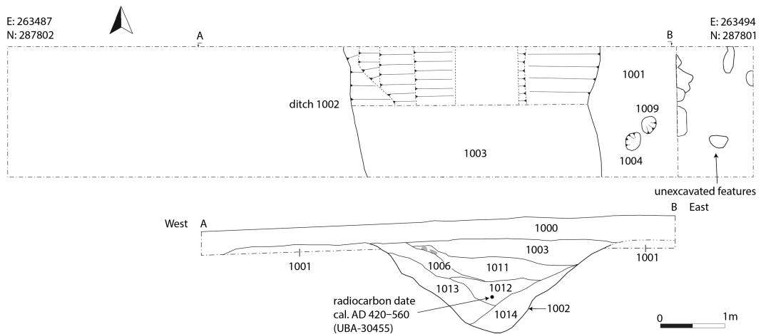
Fig. 4. Trench 1: plan and section.
