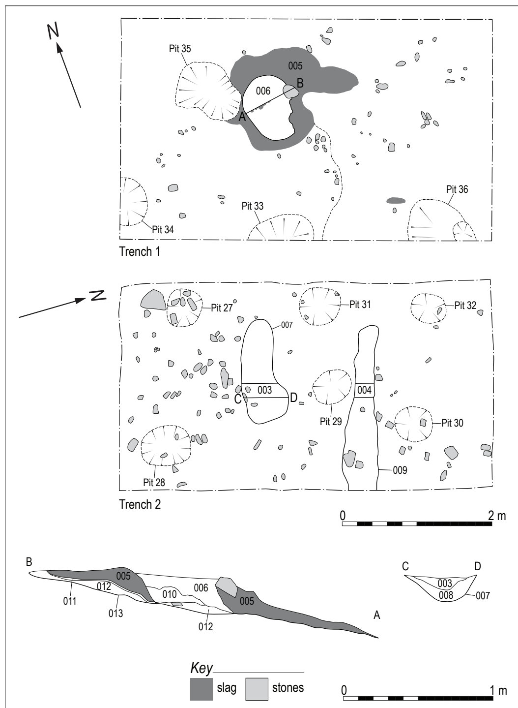
ILLUS 3 Plans of trenches 1 and 2 and east/west section through bloomery furnace
