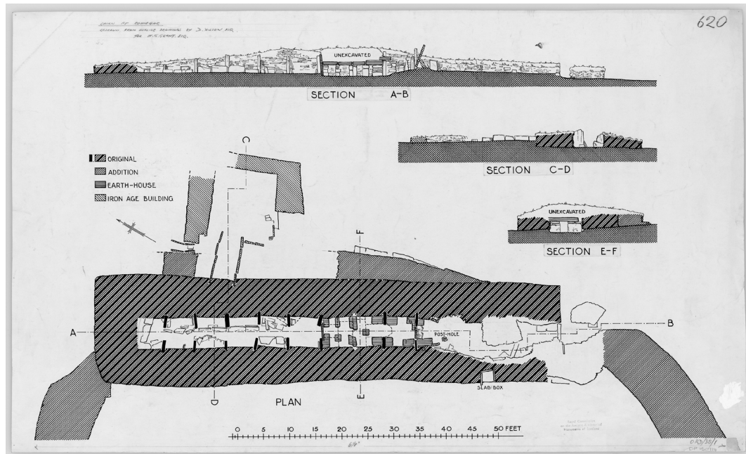
ILLUS 2 Plan and sections of the Knowe of Rowiegar. From RCHMS Inventory for Orkney (1946), attributed to W G Grant, with permission of RCAHMS
