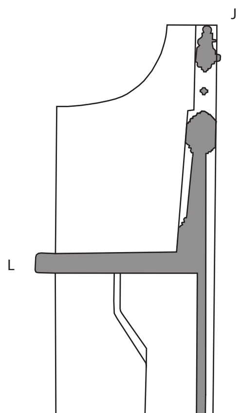
CROSS-SECTION J-K-L
