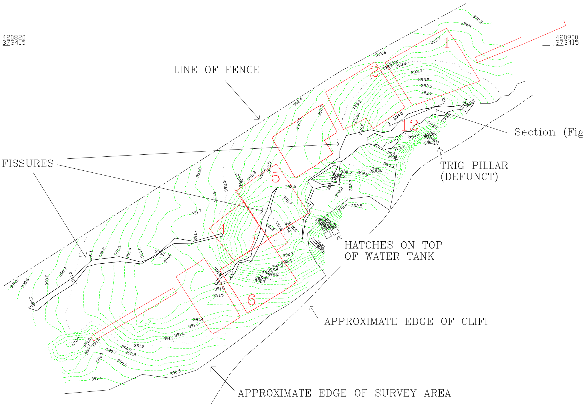
Fig 2 Contour map of Longstone Edge.
