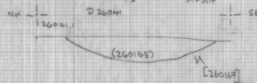
A14 TEA 26 SW facing section of ditch corner [260167] AKM 31/03/17 1:10 D 26041
