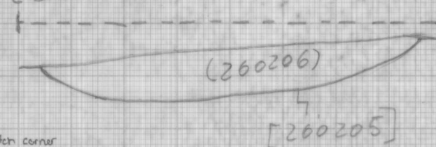
NORTH FACING SECTION OF DITCH [260205] L. 6 30/03/17 1:10 ED 26059.1 WD 26059.2
