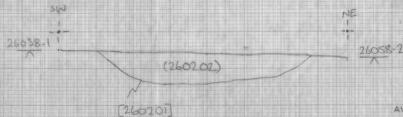
D. 26058 SE FACING SECTION OF DITCH RP 30/3/17 1:10
