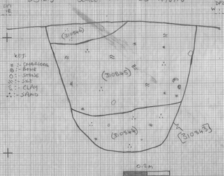
NE FACING SECTION THROUGH RINGDITCH TERMINUS [310843] D31213 SCALE: 1:10 CB 14/6/18
