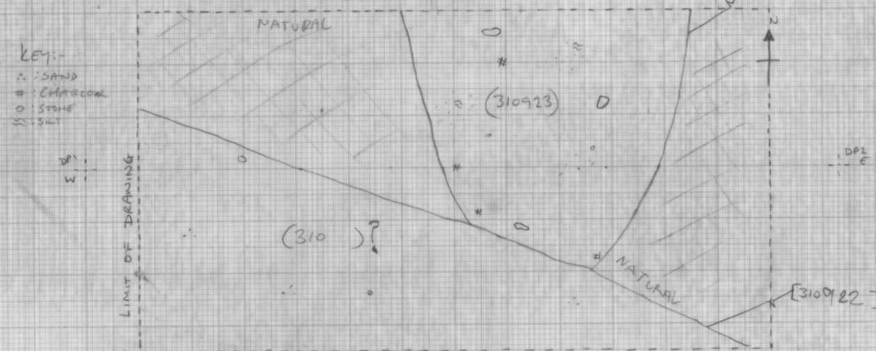
PLAN OF RELATIONSHIP BETWEEN RINGDITCH [310921] x DITCH [310922] D31224 SCALE: 1:10 CB 18/6/18
