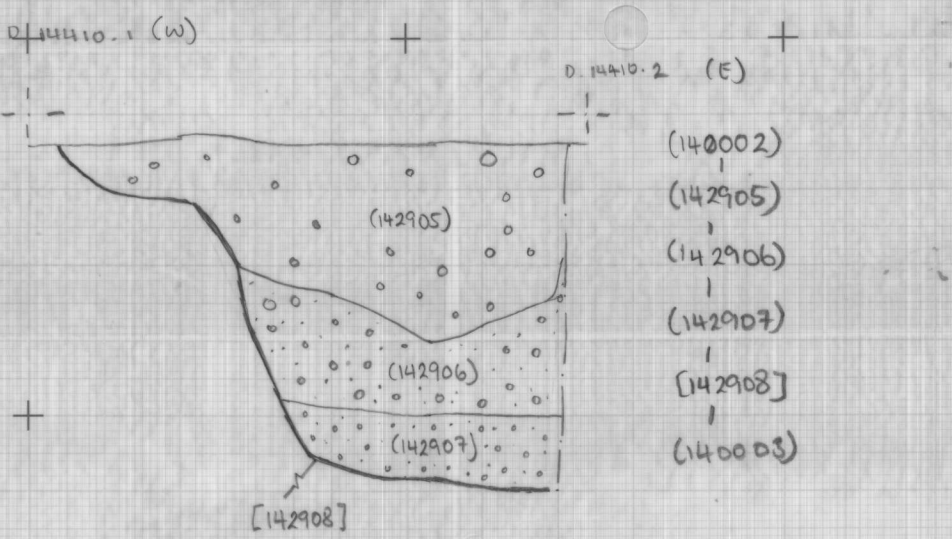
D. 14410 SCALE = 1:10 ST 07/04/17 SOUTH FACING PROFILE SECTION OF DITCH [142908]
