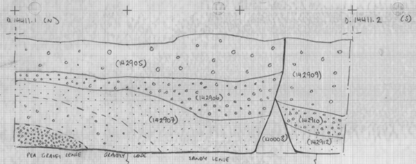
D. 14411 SCALE = 1:10 ST 07/04/17 WEST FACING RELATIONSHIP SECTION OF DITCHES [142908] AND [142912]
