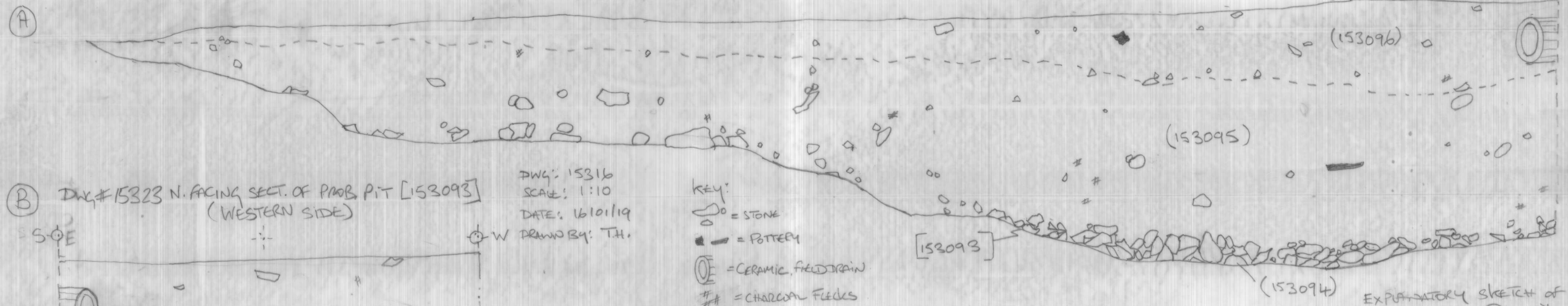
DWG# 15316 WEST-FACING SECTION OF PROBABLE PIT WITH DUMPED STONES AT BASE [153093]
