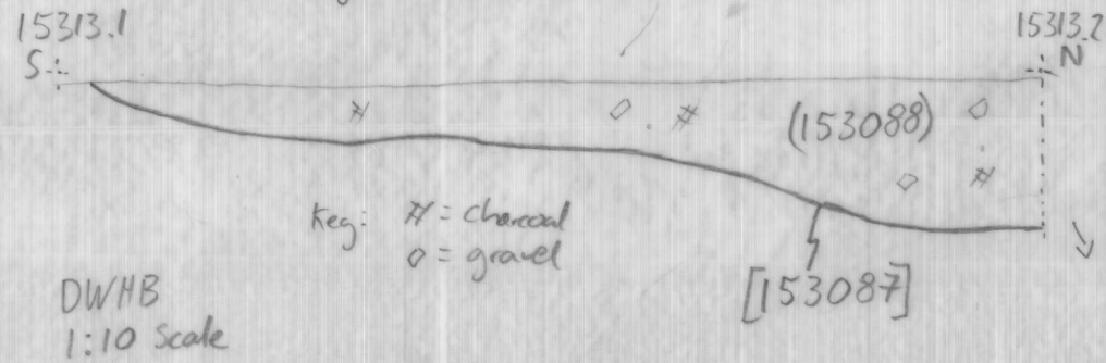
East Facing Section of Ditch Terminus D#15313
