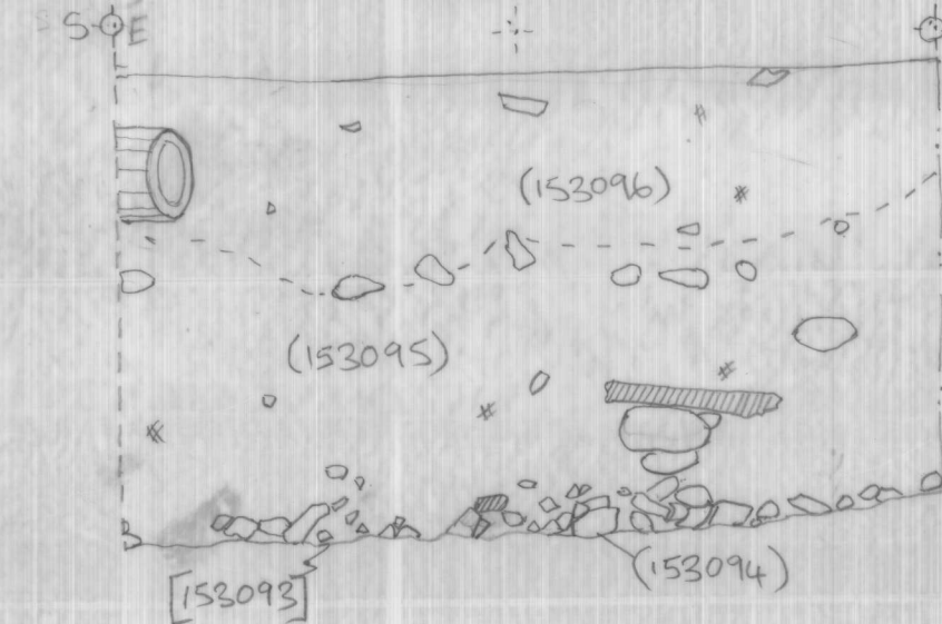
DWG# 15323 N. FACING SECT. OF PROB. PIT [153093] (WESTERN SIDE)
