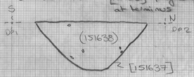
DWG #15148 [151637] profile of ditch at terminus
