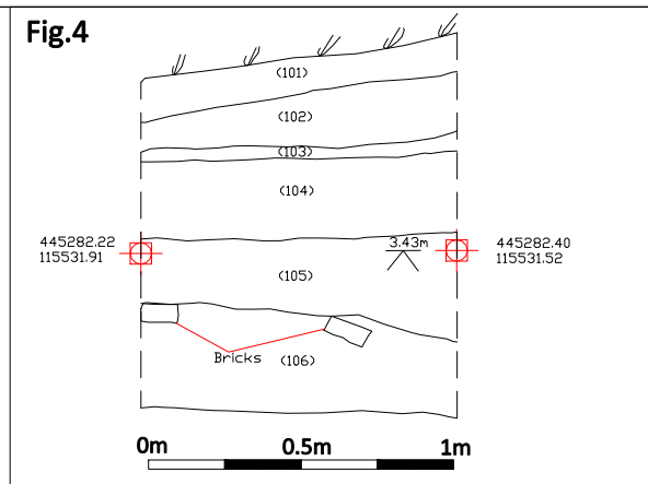
Figures 3, 4, 5, and 6: Plan of the PDA and representative sections
