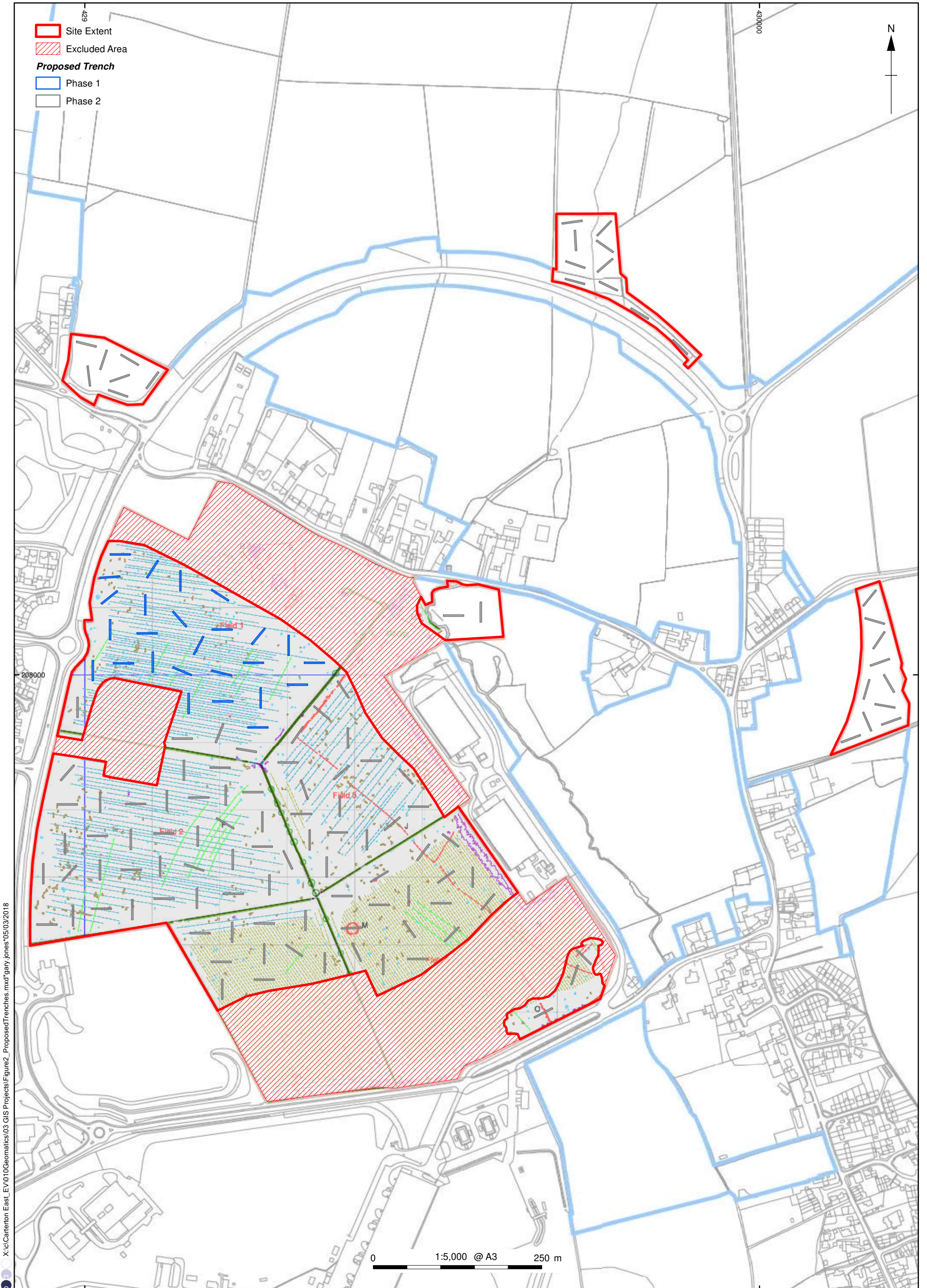
Figure 3: Proposed trench locations and geophysical survey results
