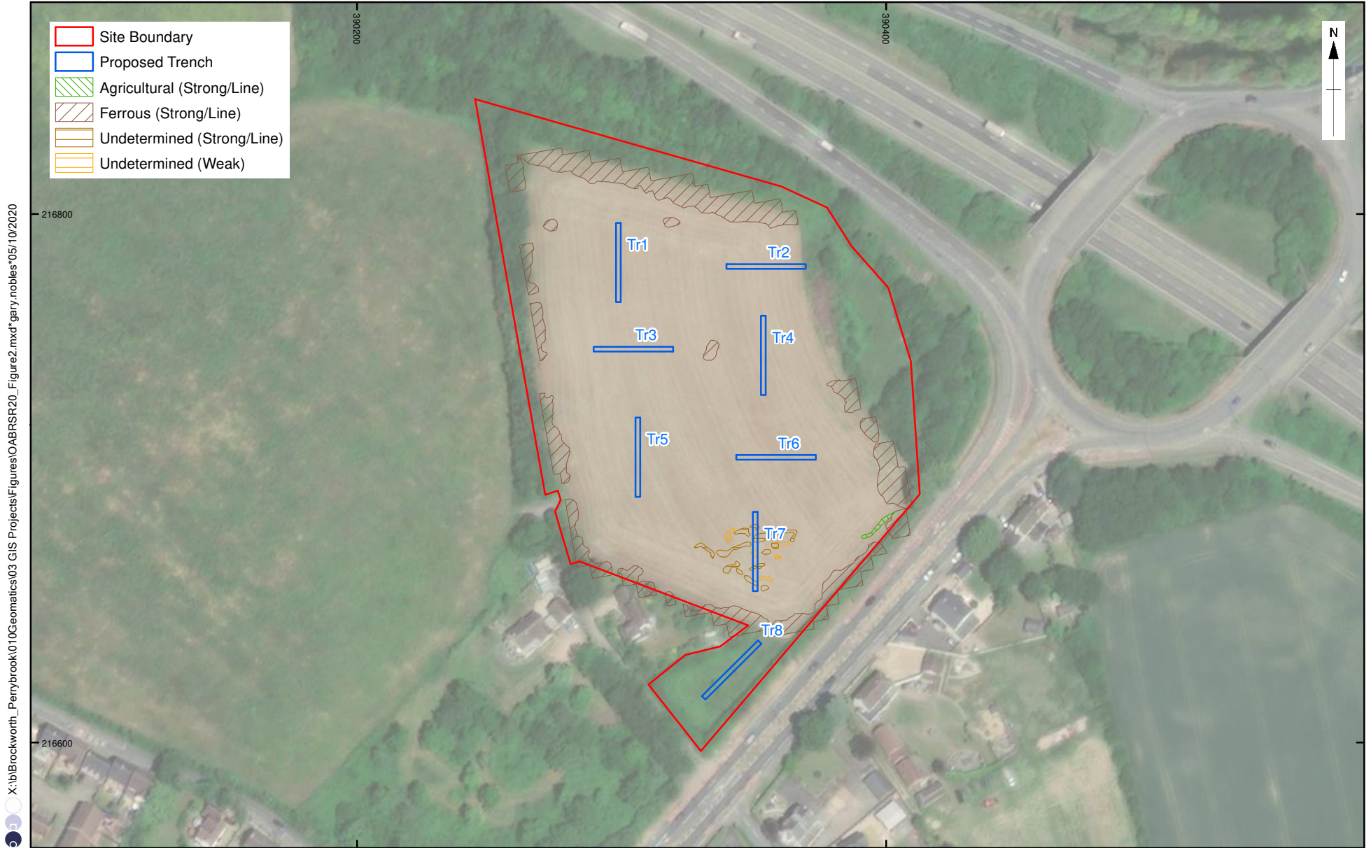
Figure 2: Proposed trench layout
