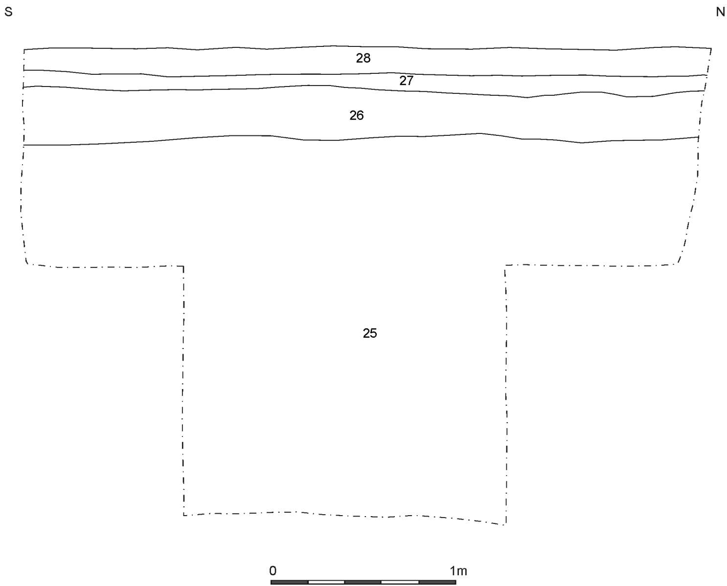
Figure 3. Trench 1, east-facing section. Scale 1:20
