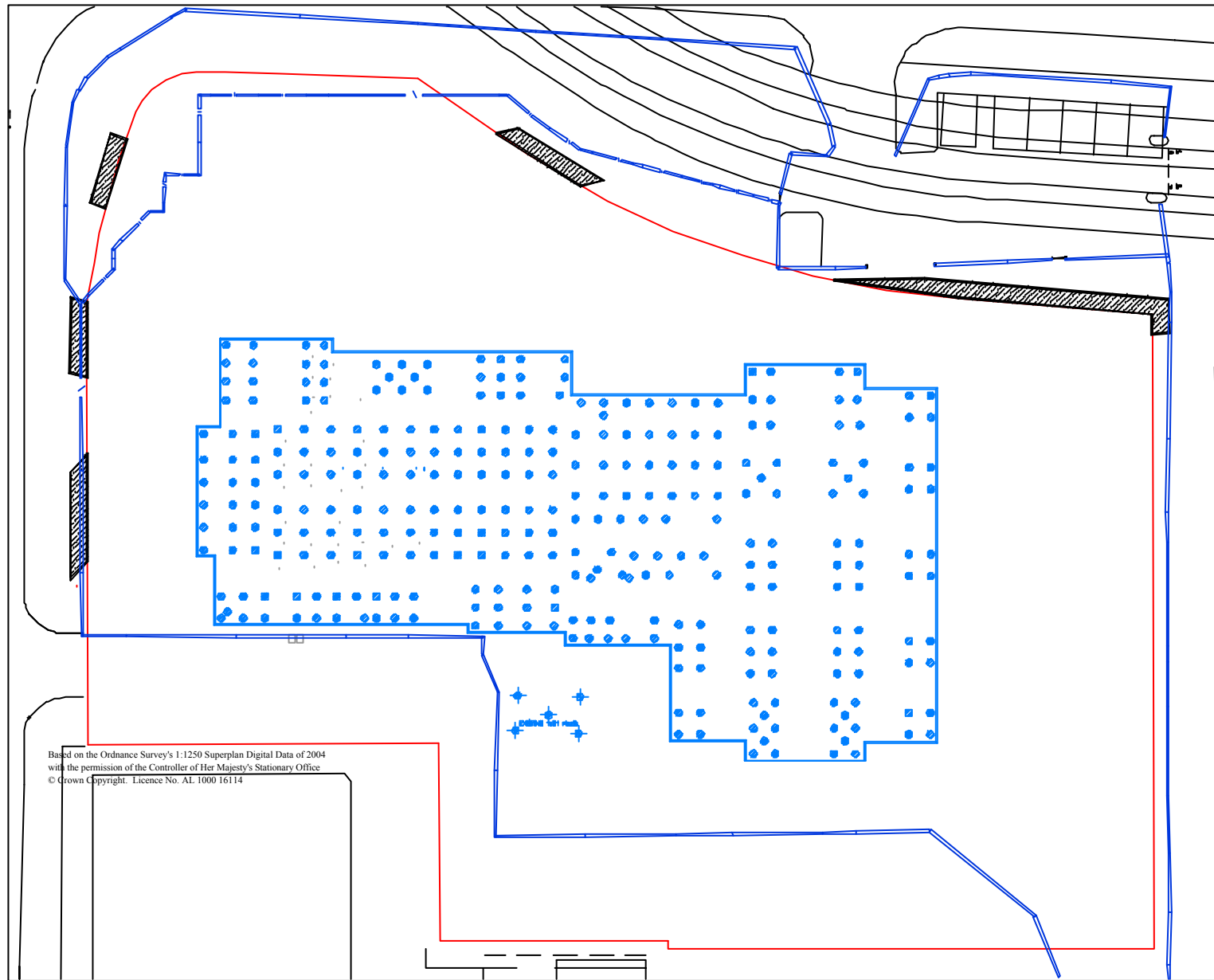
Figure 5: Footprint of Building with Piled Foundations
