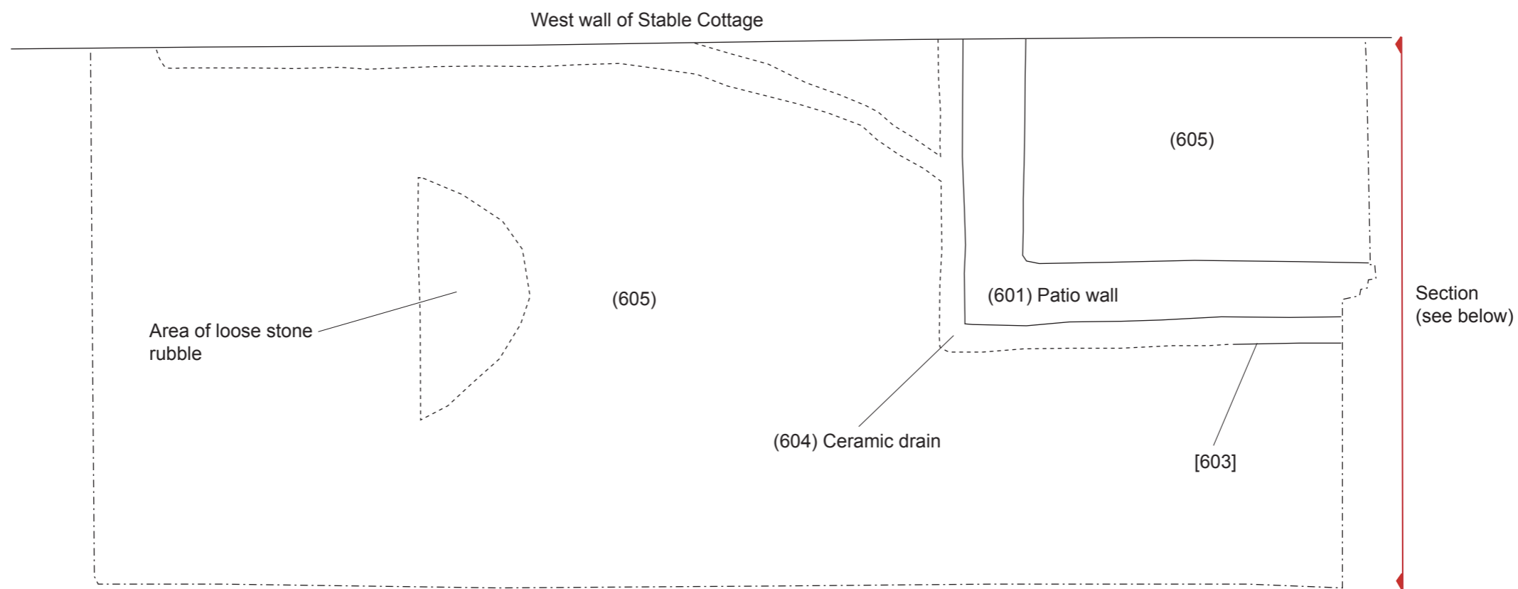
Figure 3a: Plan of Trench 6, for conservatory foundations at Stable Cottage
