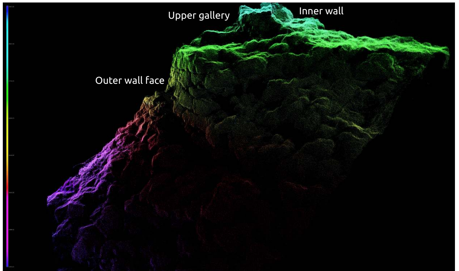
Figure 4: Perspective image coloured by elevation of the collapsed wall at Point C, showing the inner wall and upper gallery space (facing SW).
