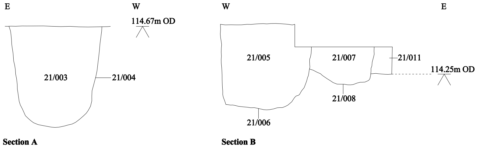
Figure 4: Ditch Sections [21/004] & [21/008]
