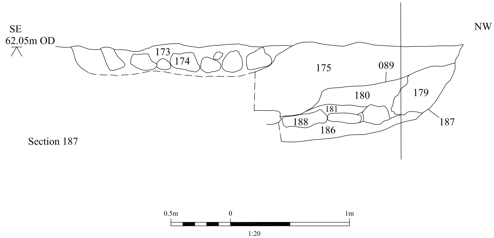
Figure 7: Section of 187
