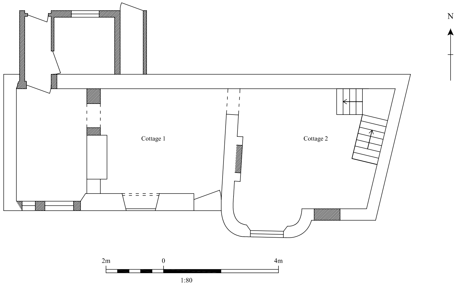
Figure 3: Ground Floor
