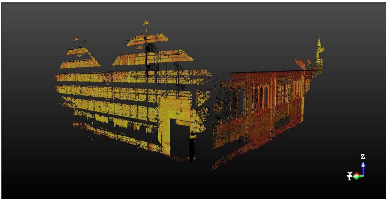
Point Cloud Data After the Scaffolding Has Been Digitally Removed
