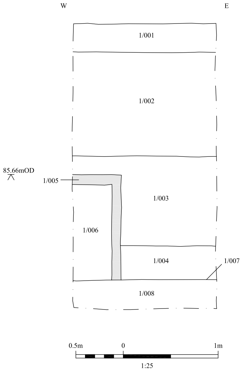
Figure 4: Sample Section from Trench 1/Service Trench
