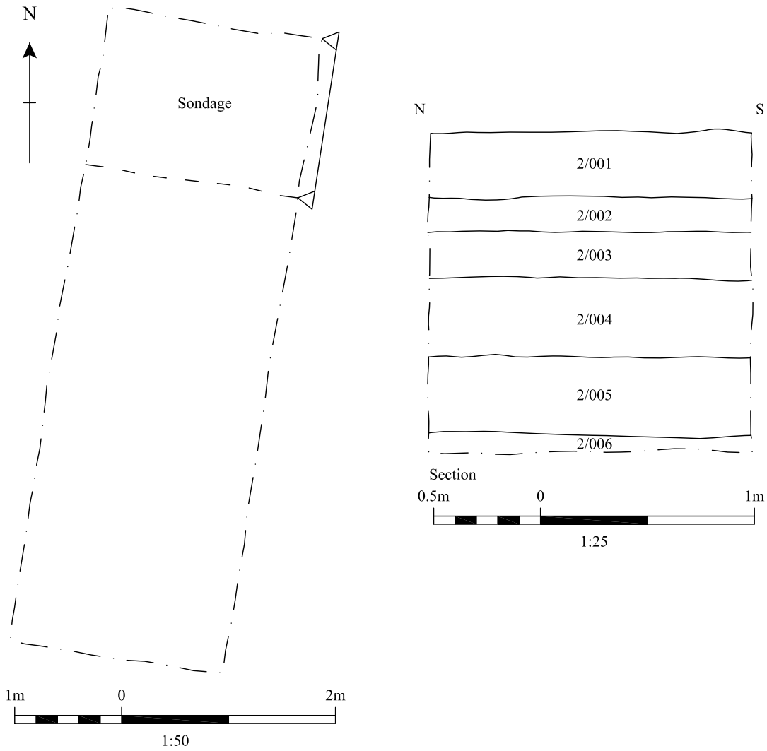
Figure 4: Trench 2: Plan (1:50) & Sample Section (1:25)
