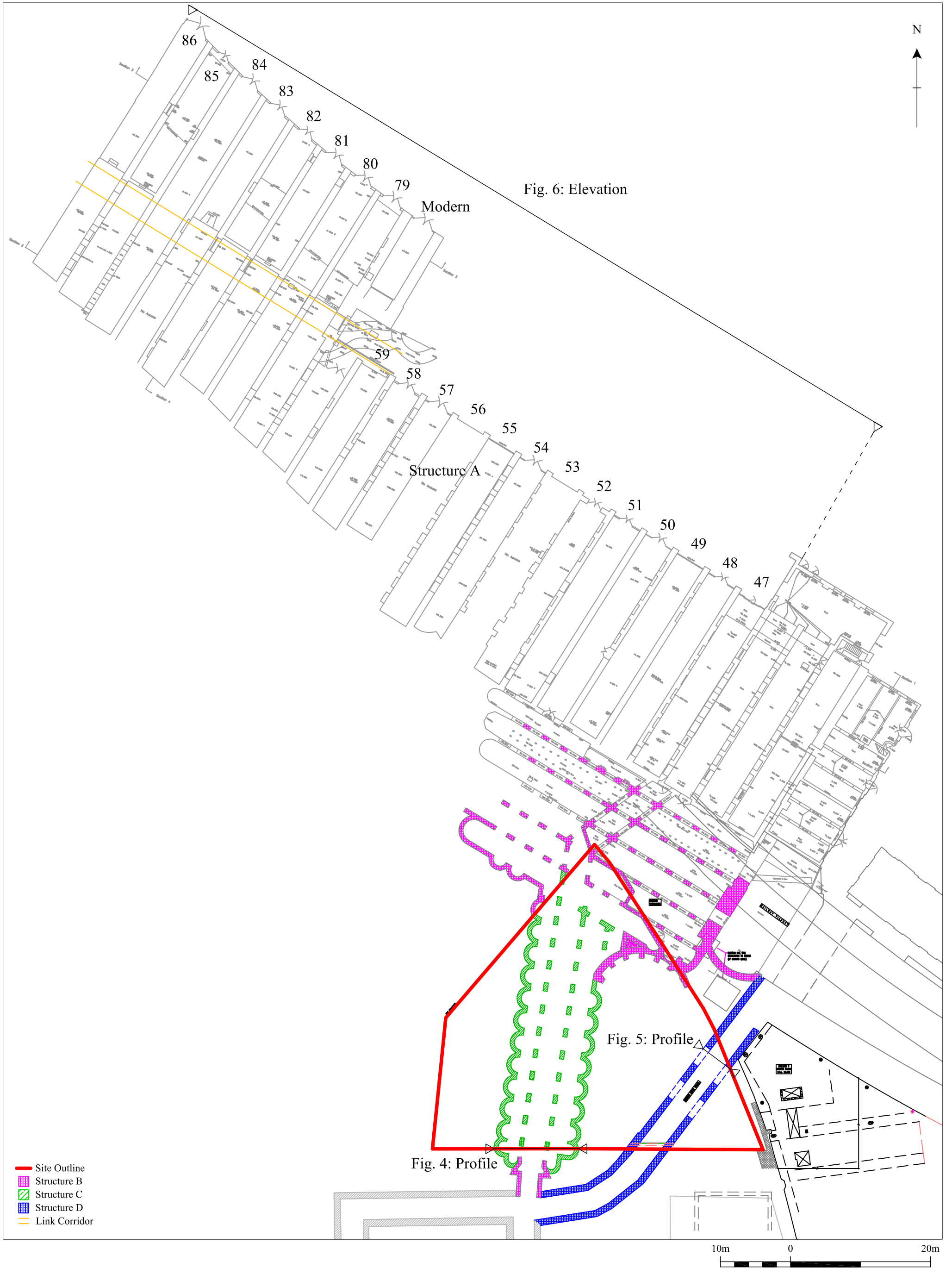
Figure 3: Plan Showing Brick Structures in the Area of Excavation and Recording
