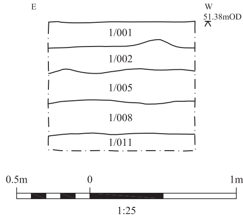
Trench 1: Section
