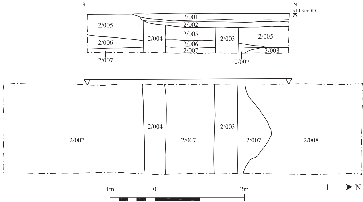
Trench 2: Plan and Section
