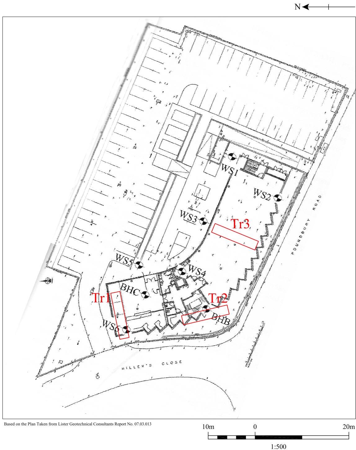
Figure 3: Trench Location Plan
