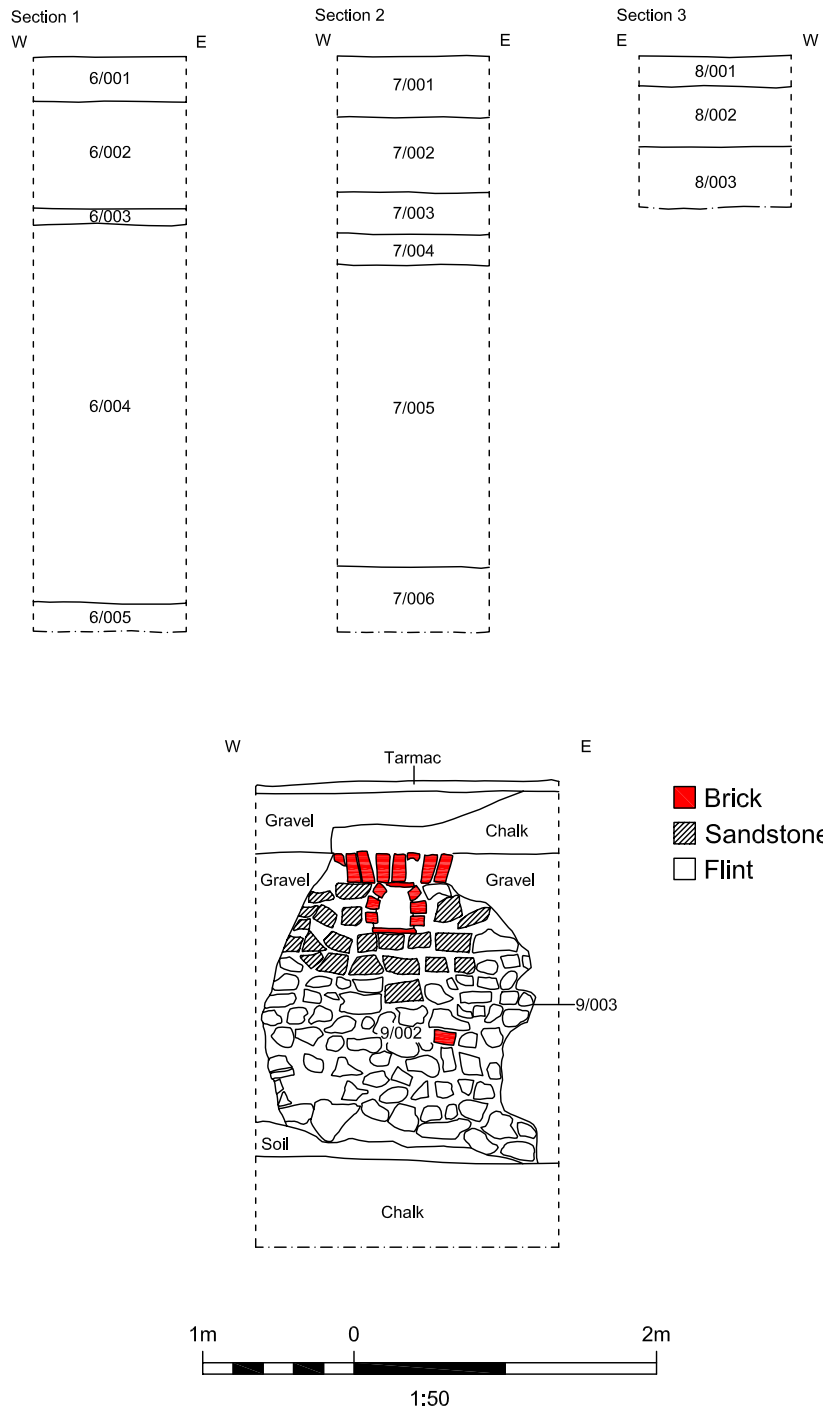
Figure 4: Sample Sections
