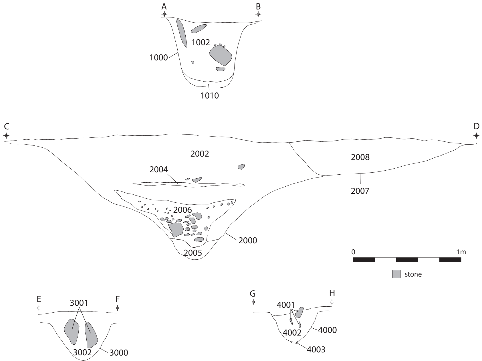
Figure 5: Sections through ditch and palisades
