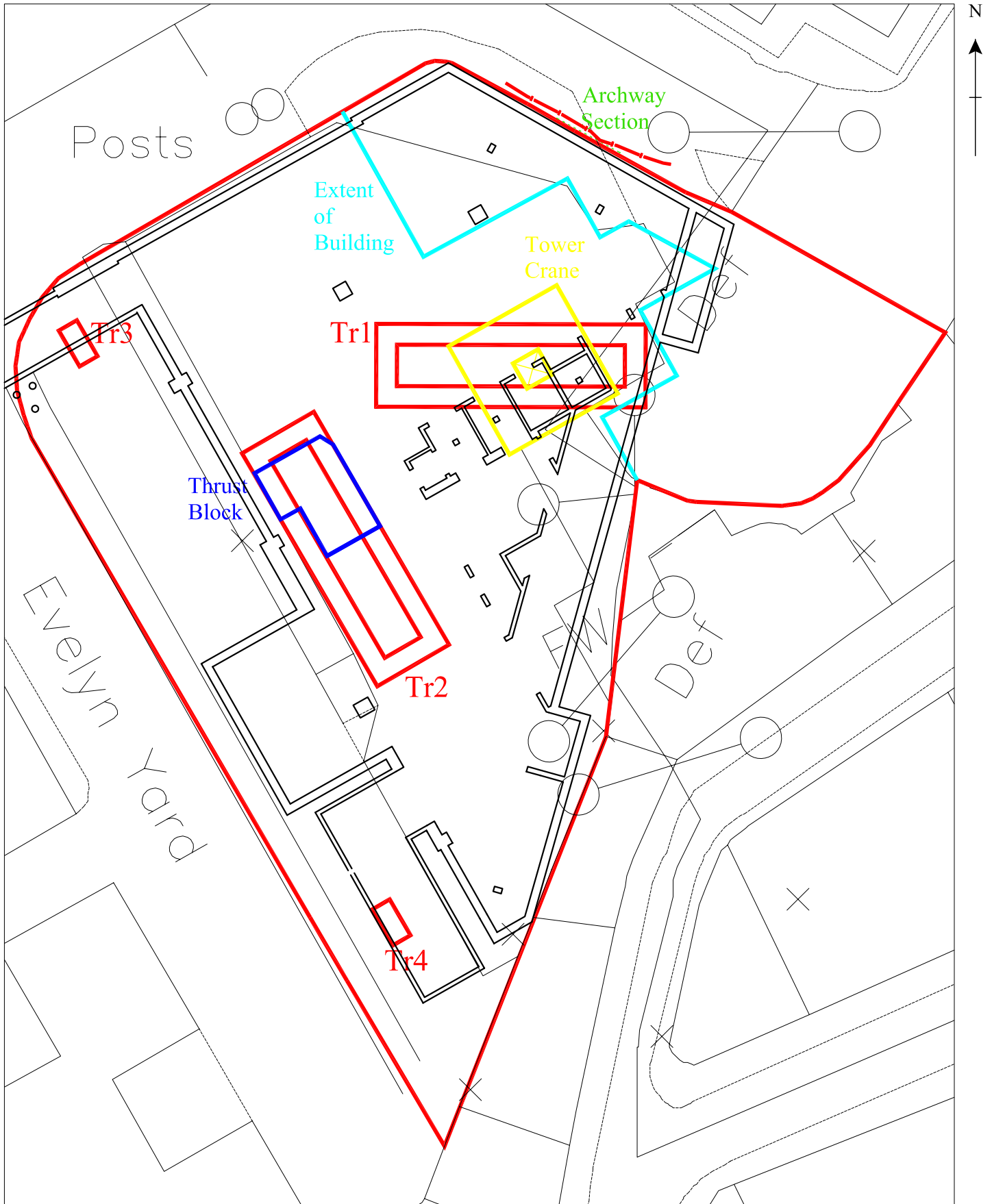
Figure 3: Trench Locations
