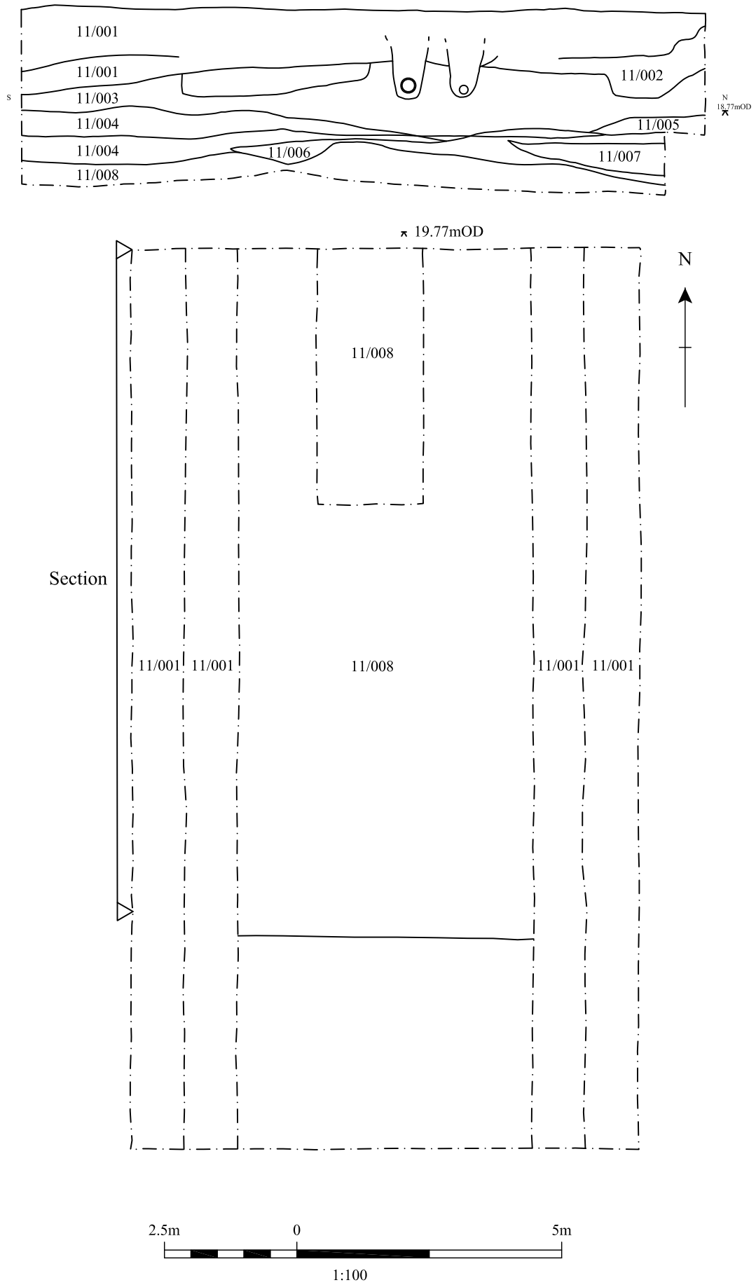
Figure 5: Trench 1: Plan and Section
