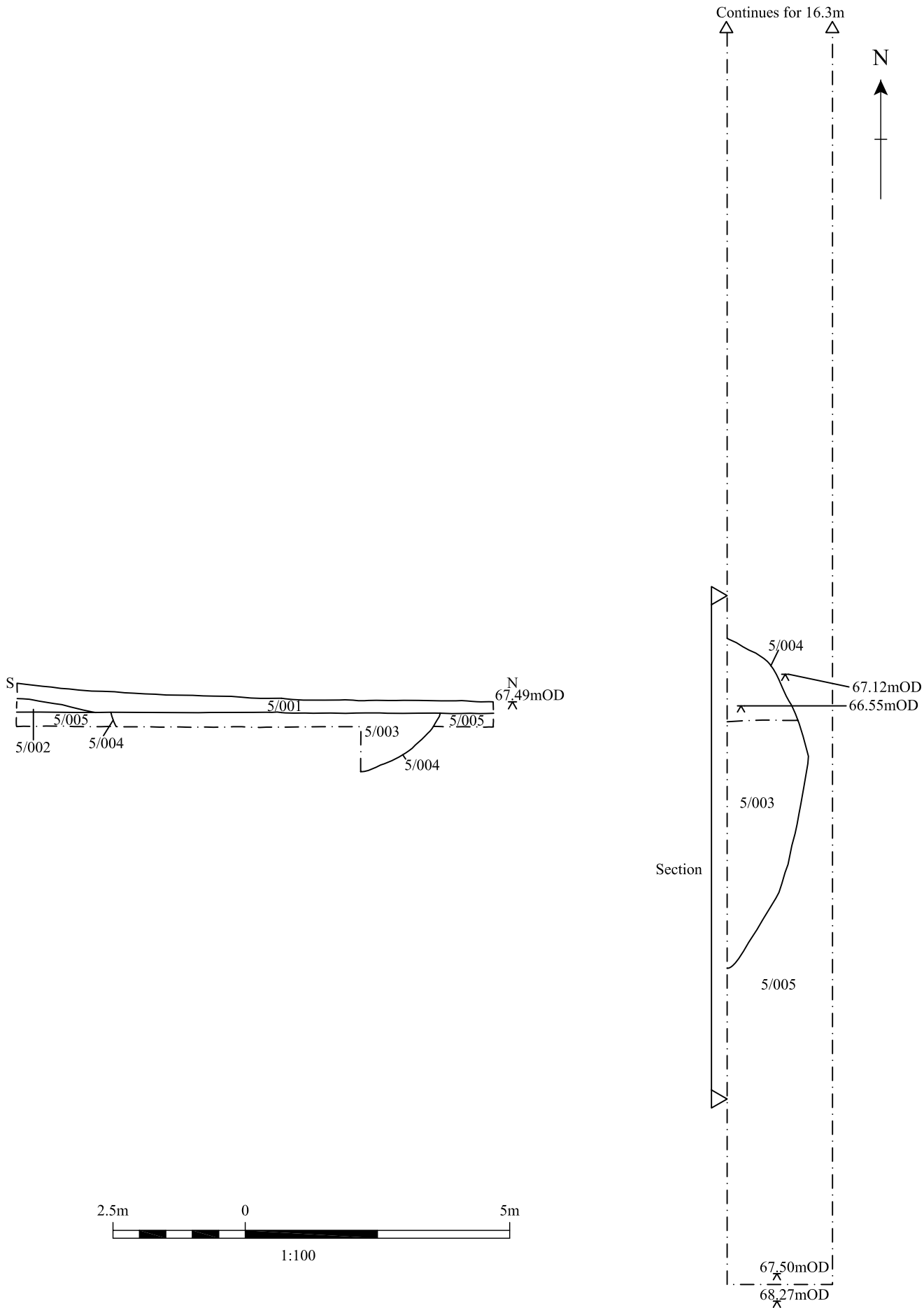
Figure 5: Trench 5: Plan & Section (1:100)
