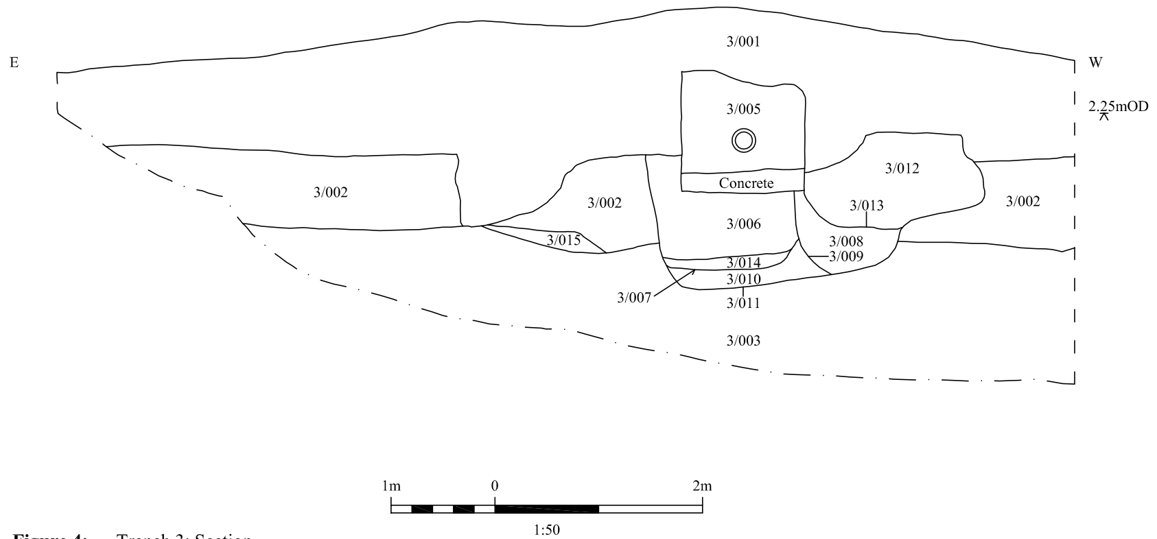
Figure 4: Trench 3: Section
