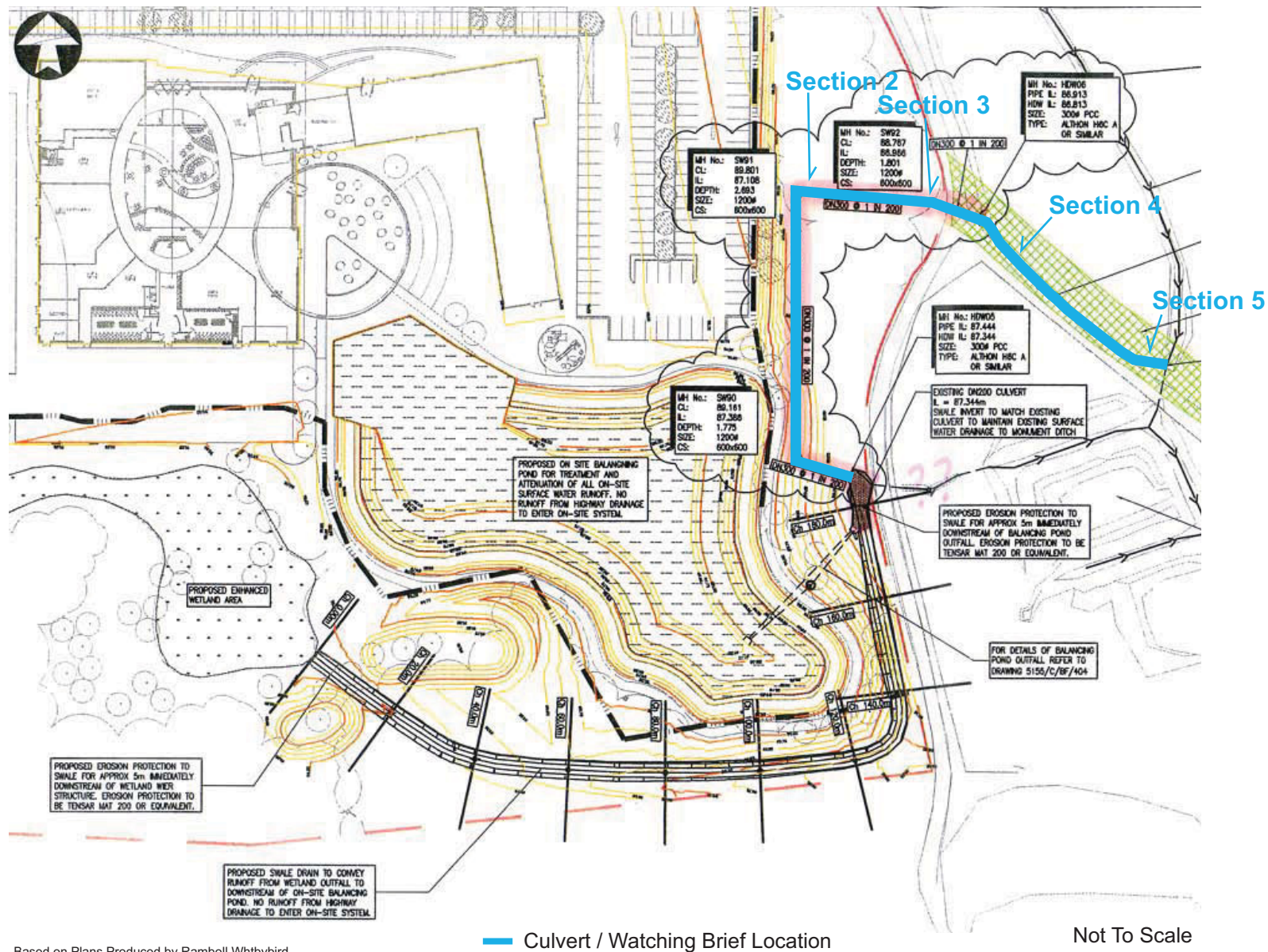
Figure 3: SWALE / Drainage Area Detail Showing Sample Section Location
