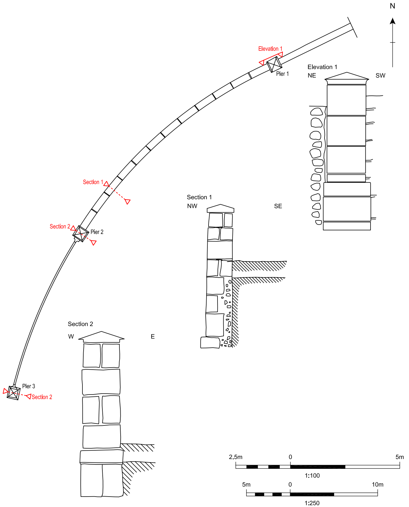
Figure 3: Boundary Wall: Plan (1:100) and Pillar Sections & Elevations (1:25)
