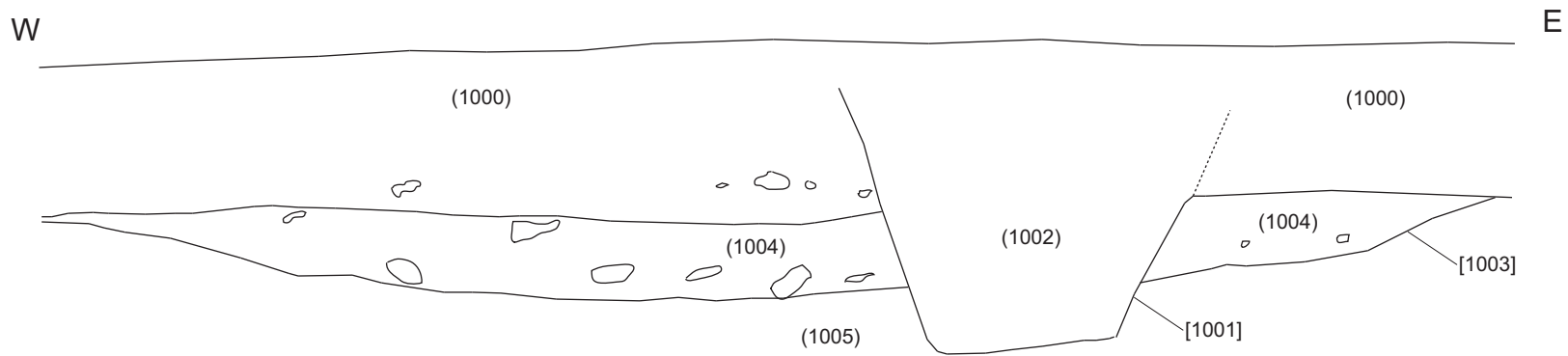
Figure 7a: South facing section through feature [1003]
