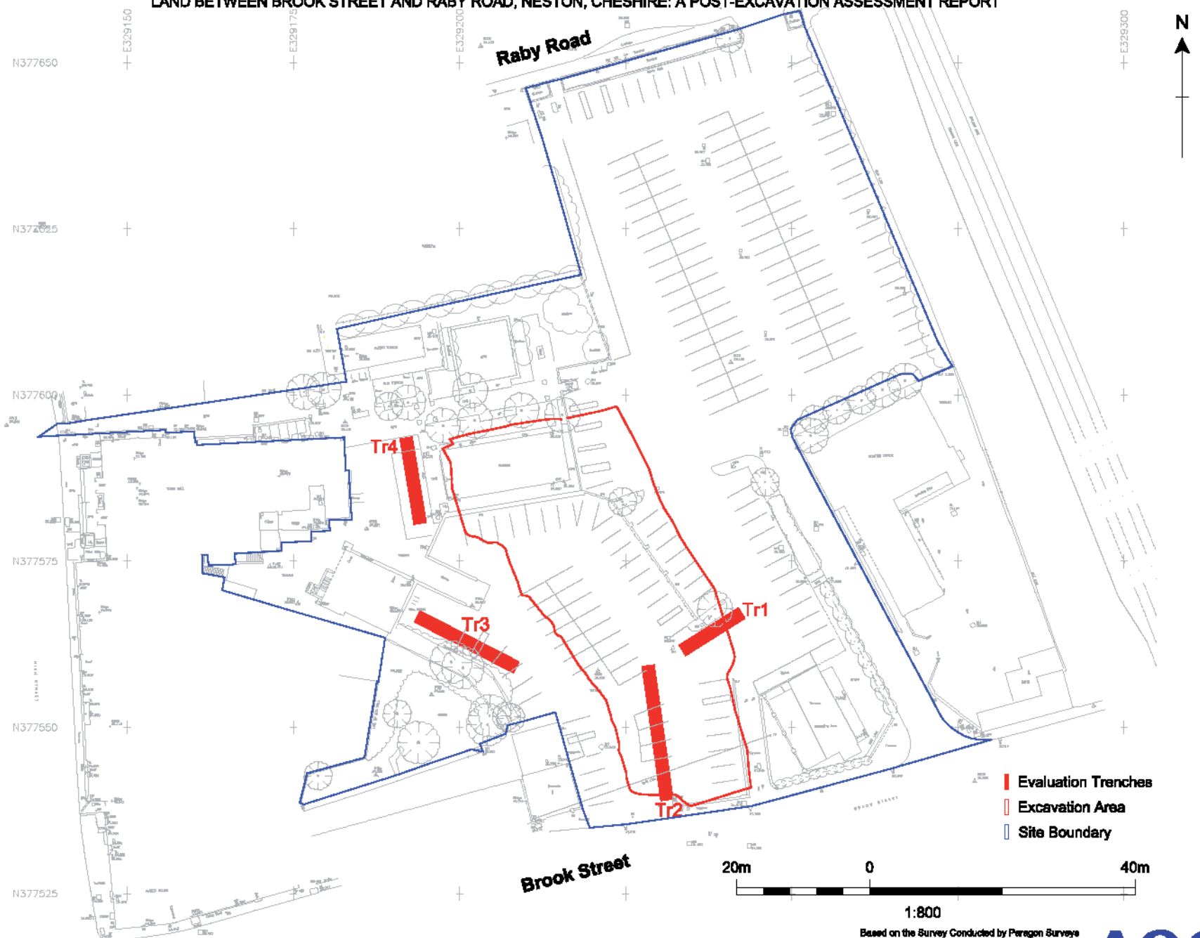
Figure 2: Evaluation Trench & Excavation Location Plan
