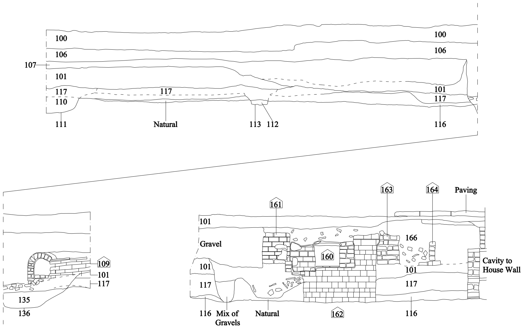
Figure 4: East Facing Section Showing Culverts
