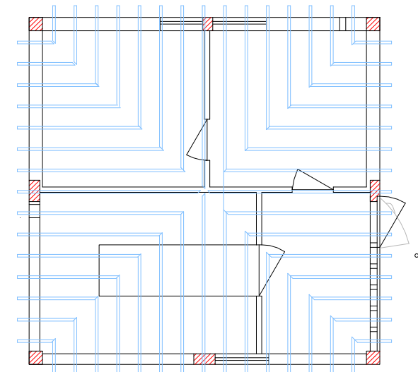
Rafters
