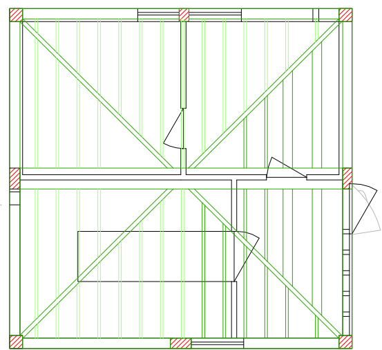
Joists
