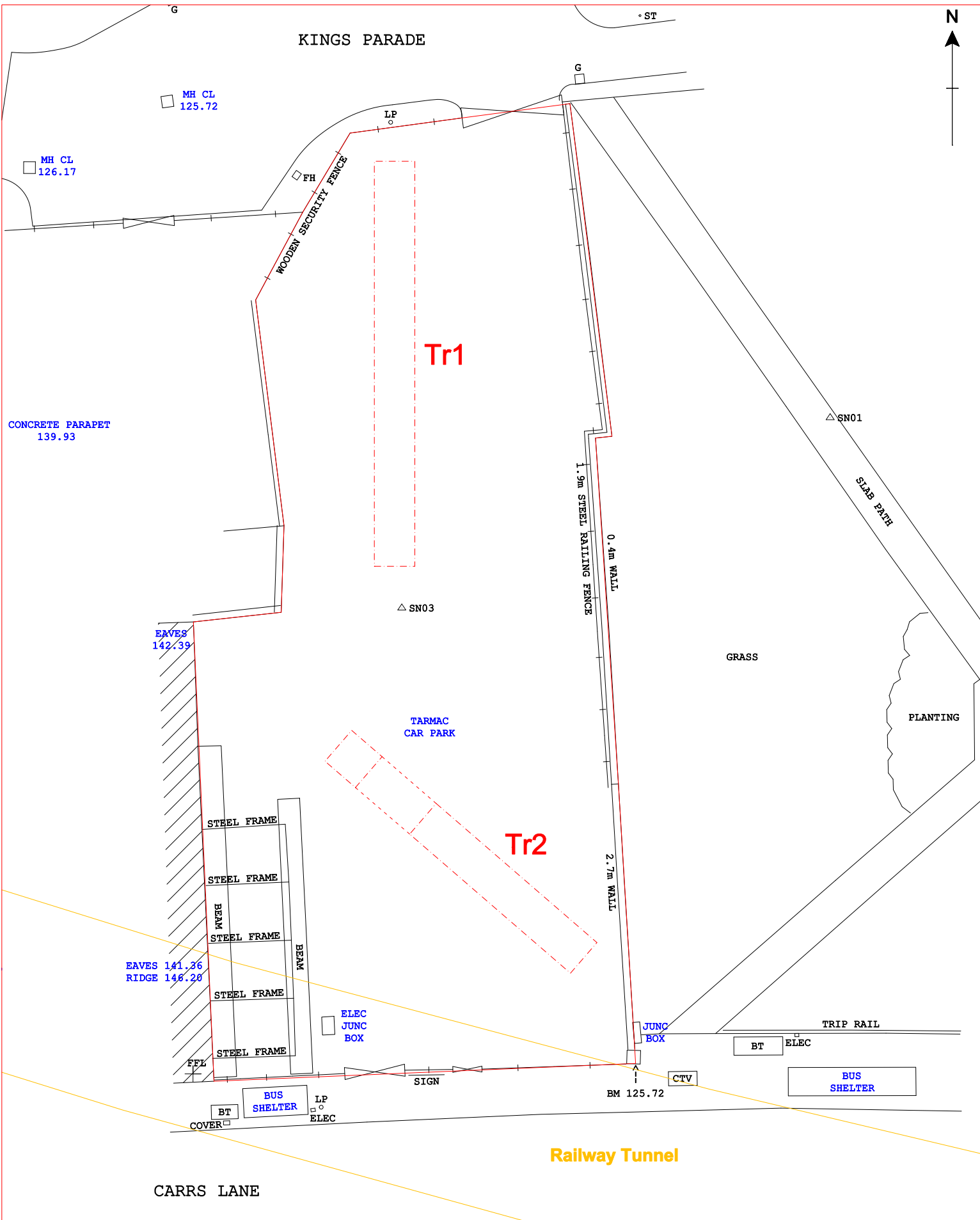
Figure 2: Detailed Site Location Plan
