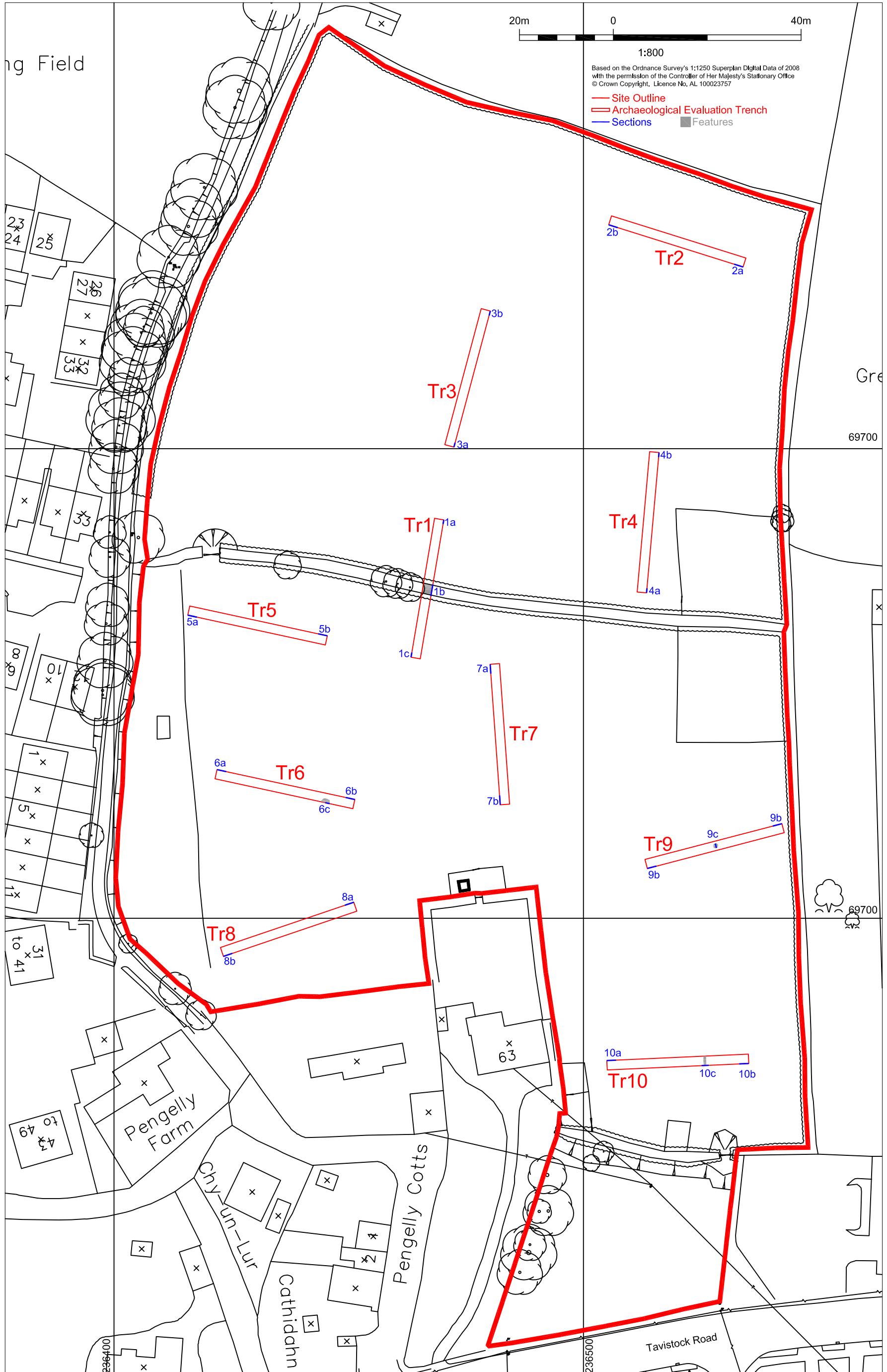
Figure 3: Detailed Feature and Section Location Plan
