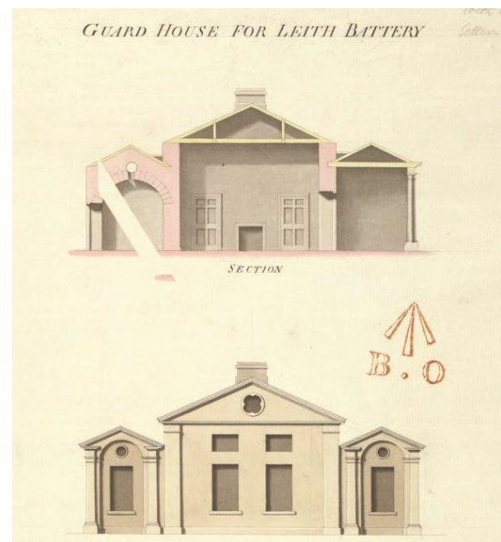
Illus 14: Guard House Section and Elevation (Watt pre-1804)
