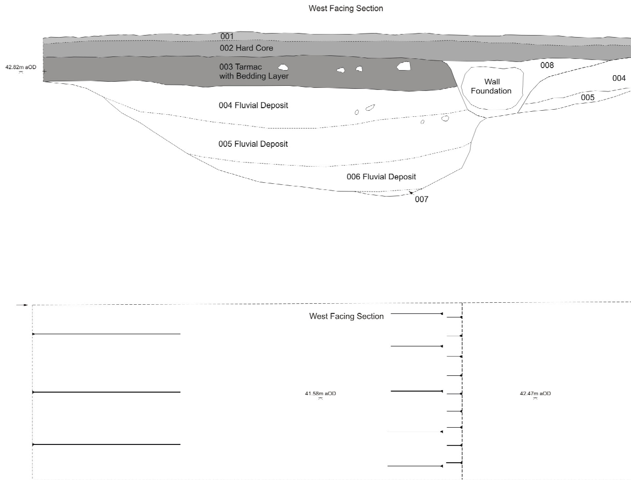
Plan and Section of Evaluation Trench One
