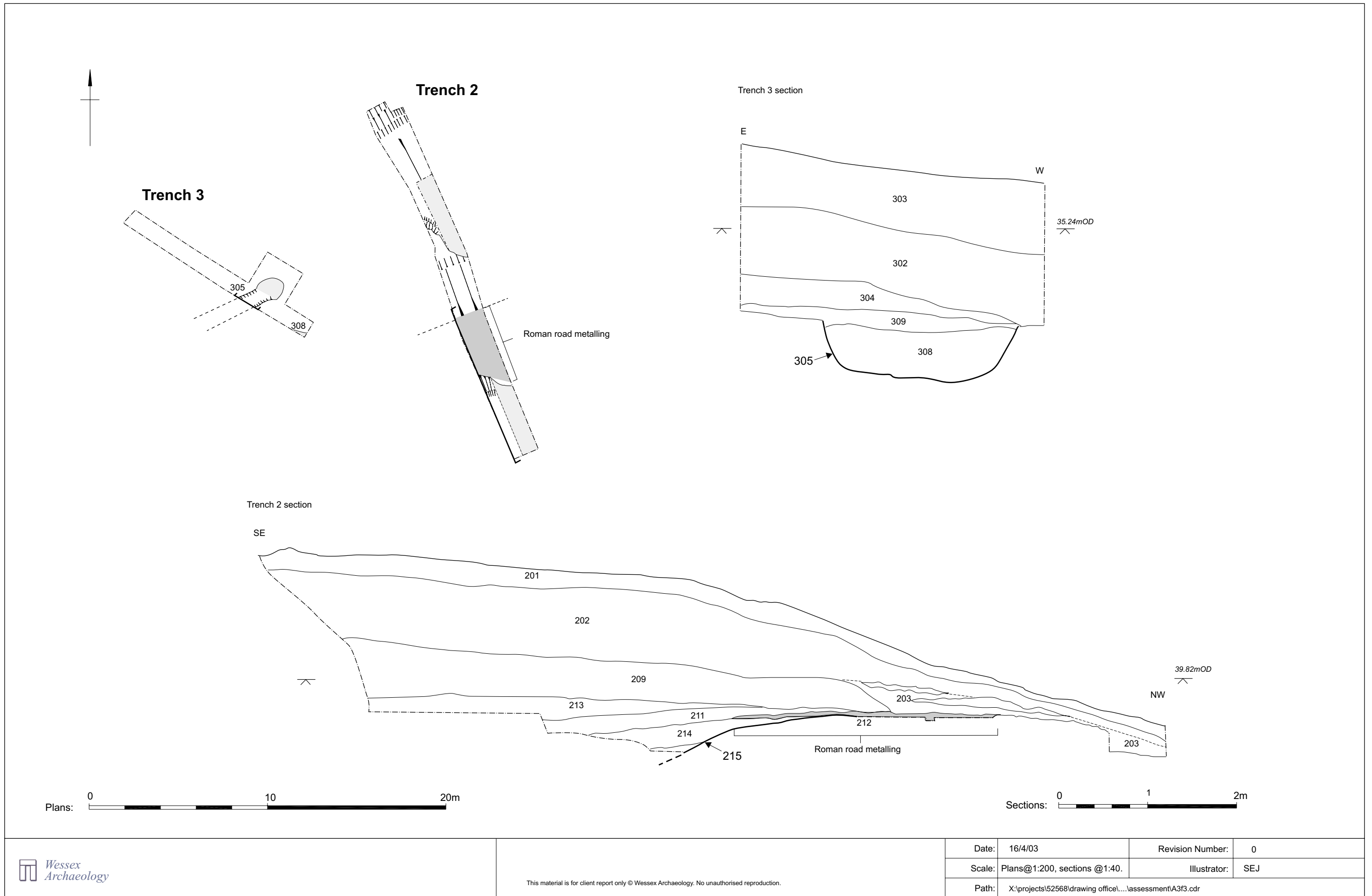
Trenches 2 and 3: Plans and sections.
