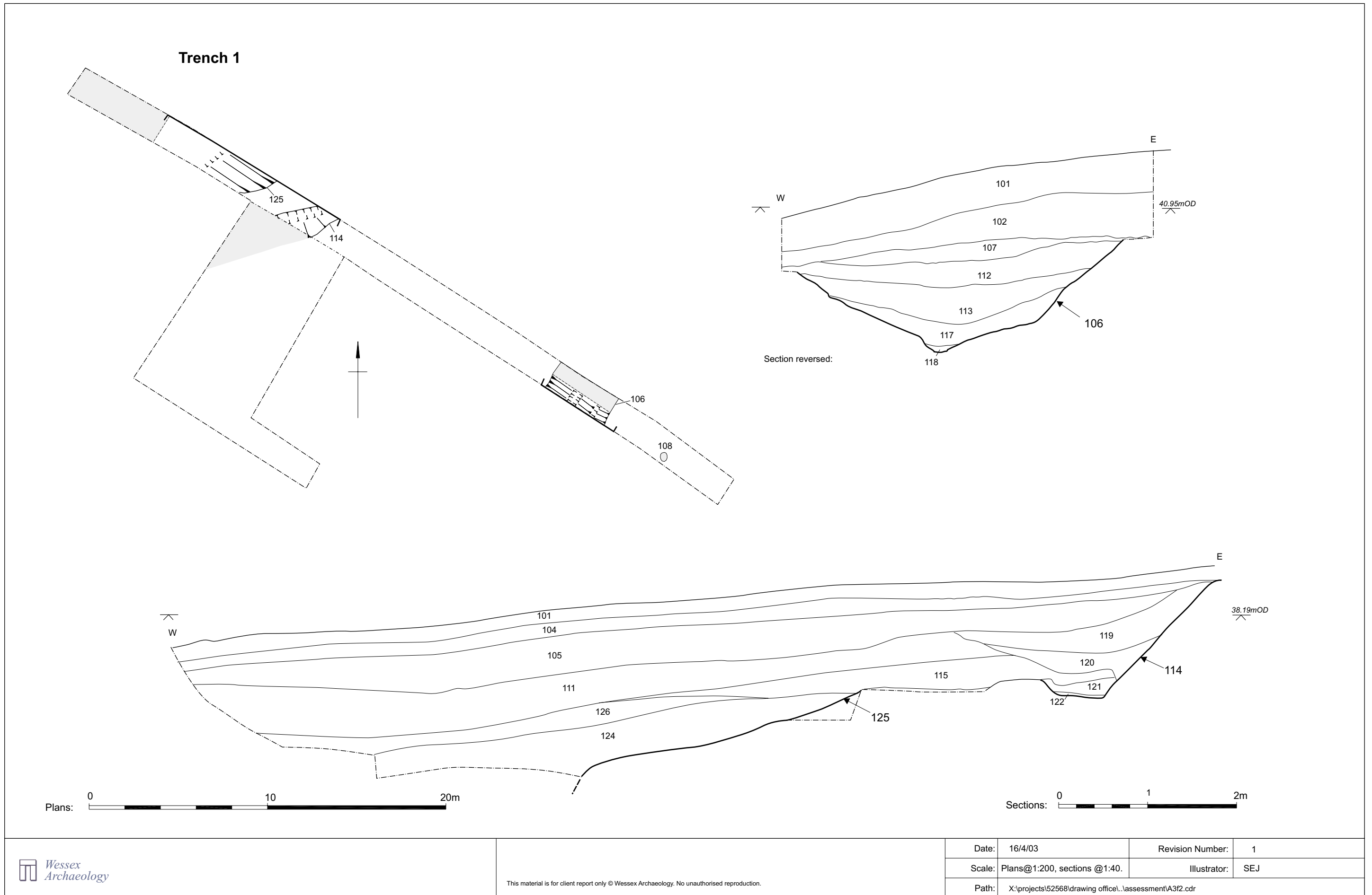
Trench 1: Plan and sections.
