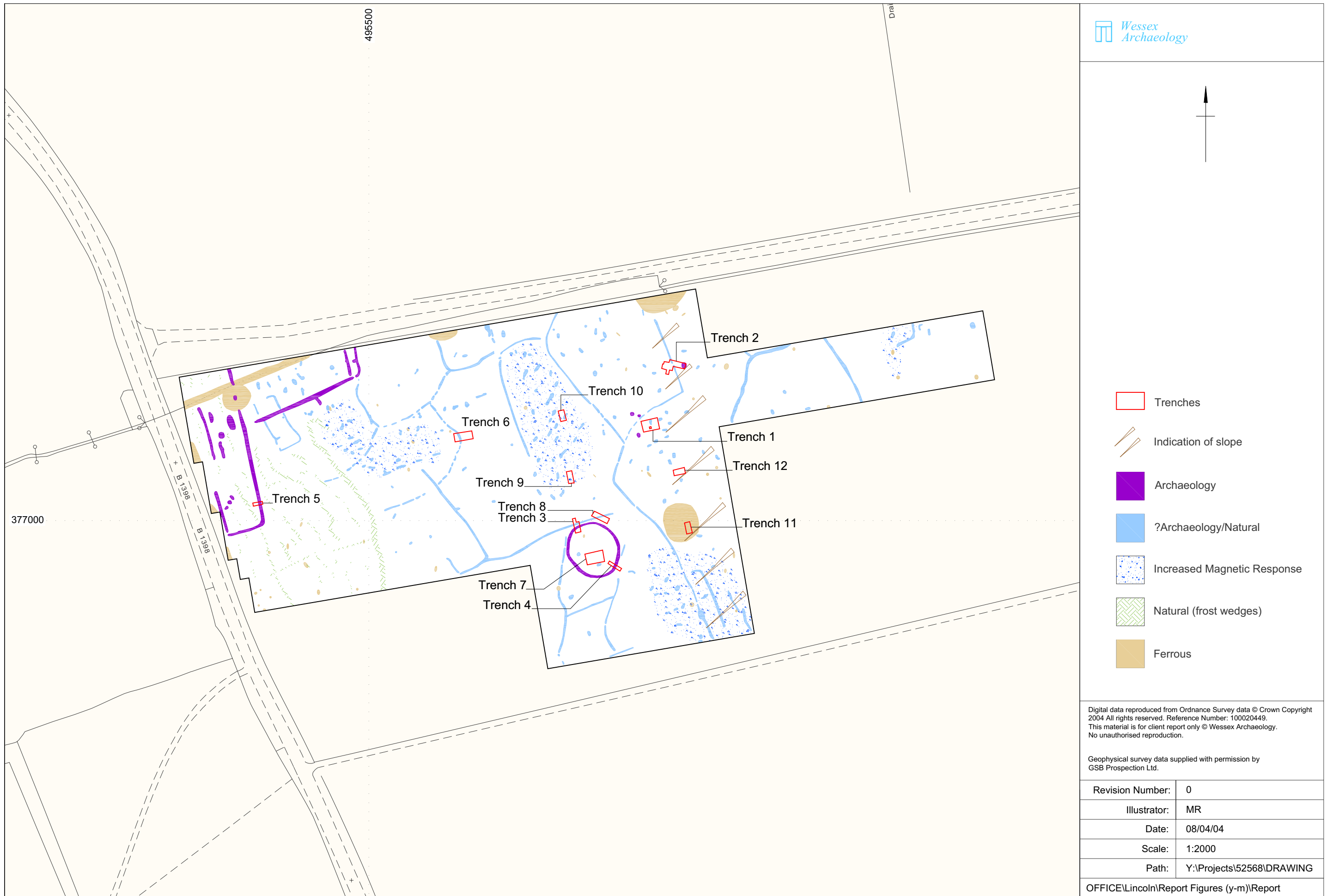
Geophysical survey results and trench location plan
