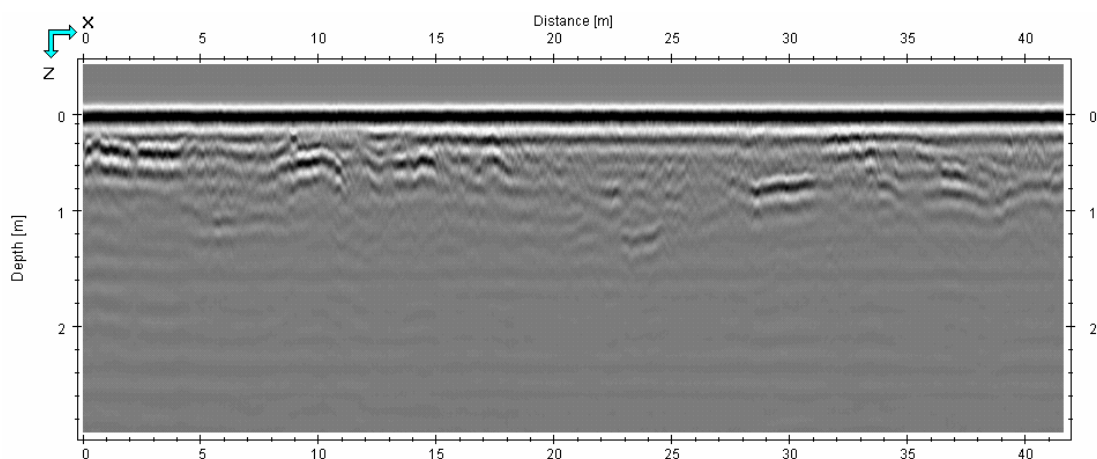
Area A profile 10046, 23m from North end of survey, shown East to West. Slightly further south than the above example, the probable track surface is evident between 28-31m.
