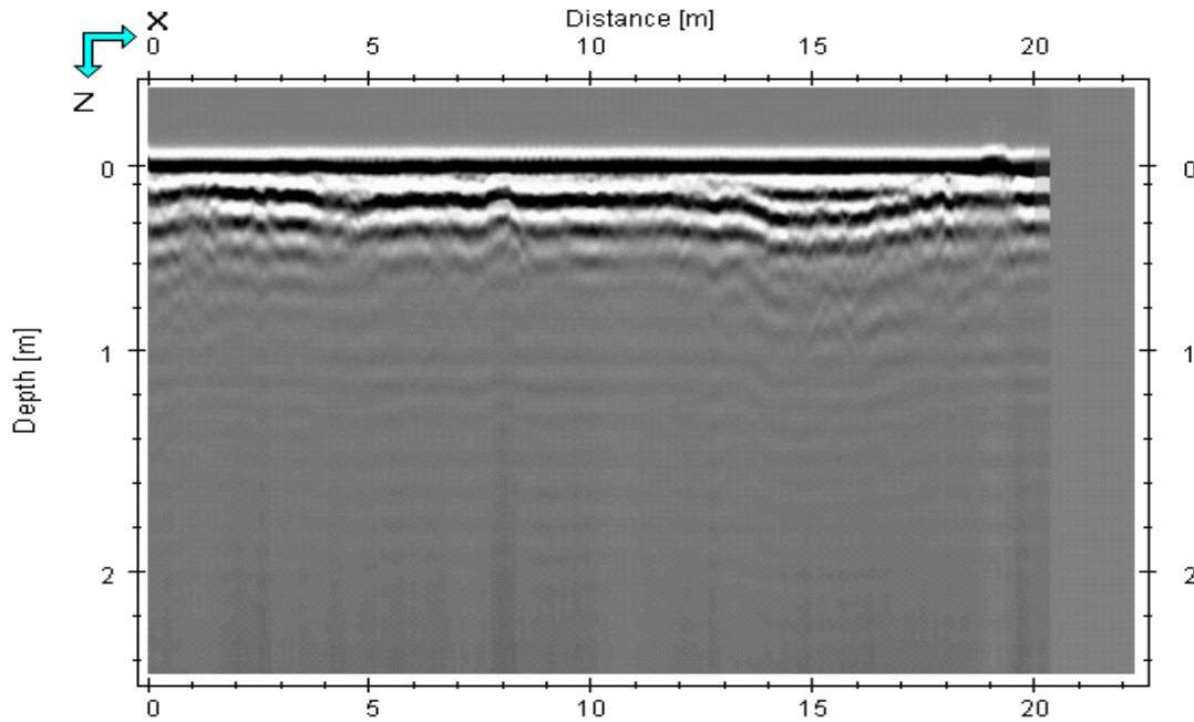
Area B profile 20077, 38m from West end of survey, shown North to South. An apparent shallow depression at around 15m is very near-surface, likely to be within the make-up of the road; the existing kerb is at 19m.
