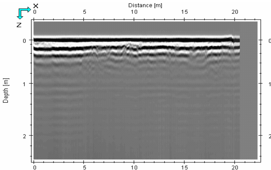
Area B profile 20105, 52m from West end of survey, shown North to South. Many small hyperbolic responses, point reflectors, reflect individual items within the road make-up; the existing kerb is at almost 20m.
