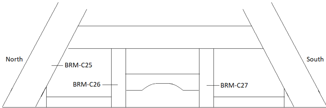
Figure 5: Schematic drawing of truss 2, showing the location of samples BRM-C25–27
