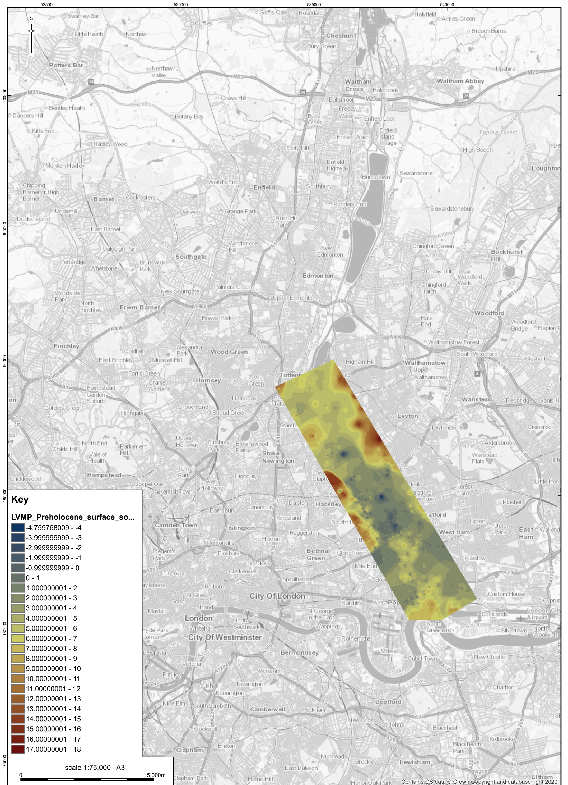
LVMP_Preholocene_surface_southern_study_area_m_OD.tif
