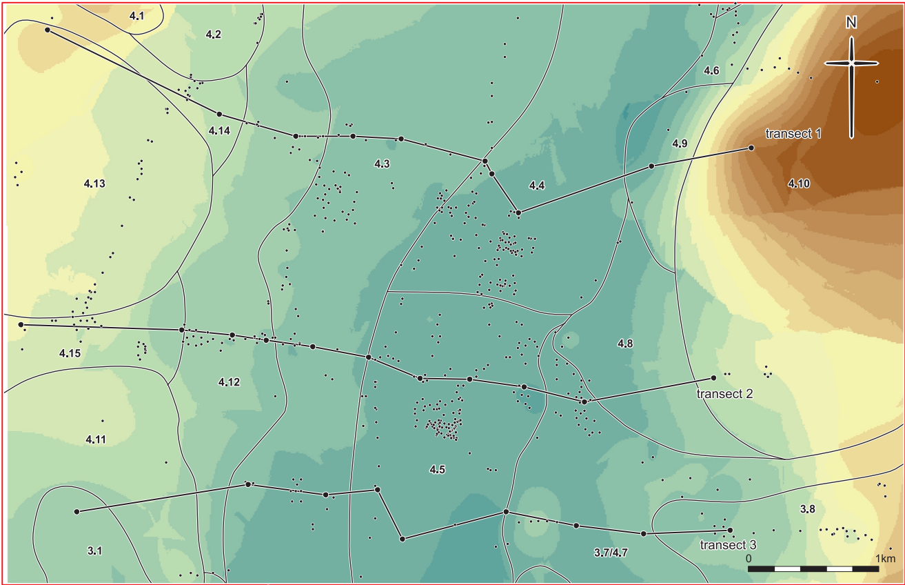
Early Holocene topography
